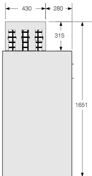
Busbar cover
