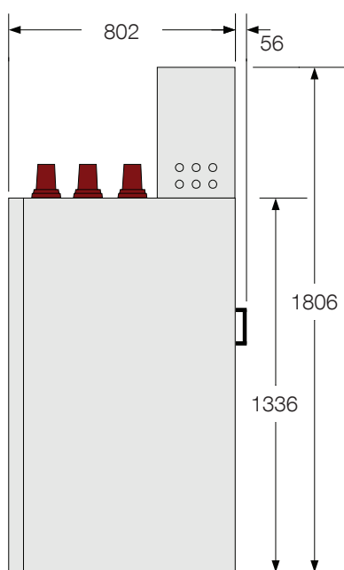
Metering module M, side view right
