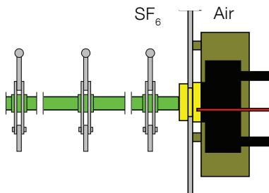
C-mechanism
