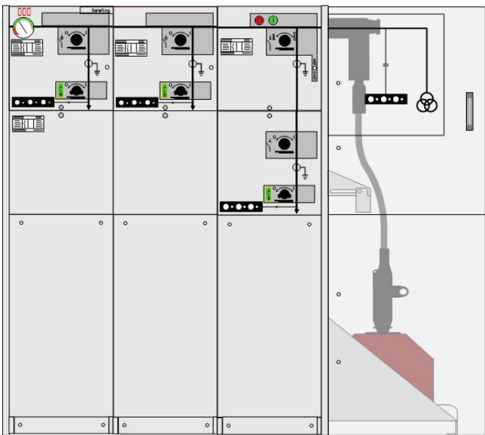
Side connected metering
