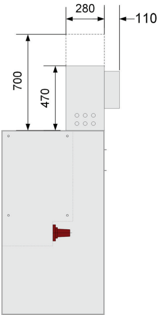
Low voltage compartment with relay type REF541
