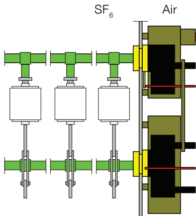
V-mechanism
